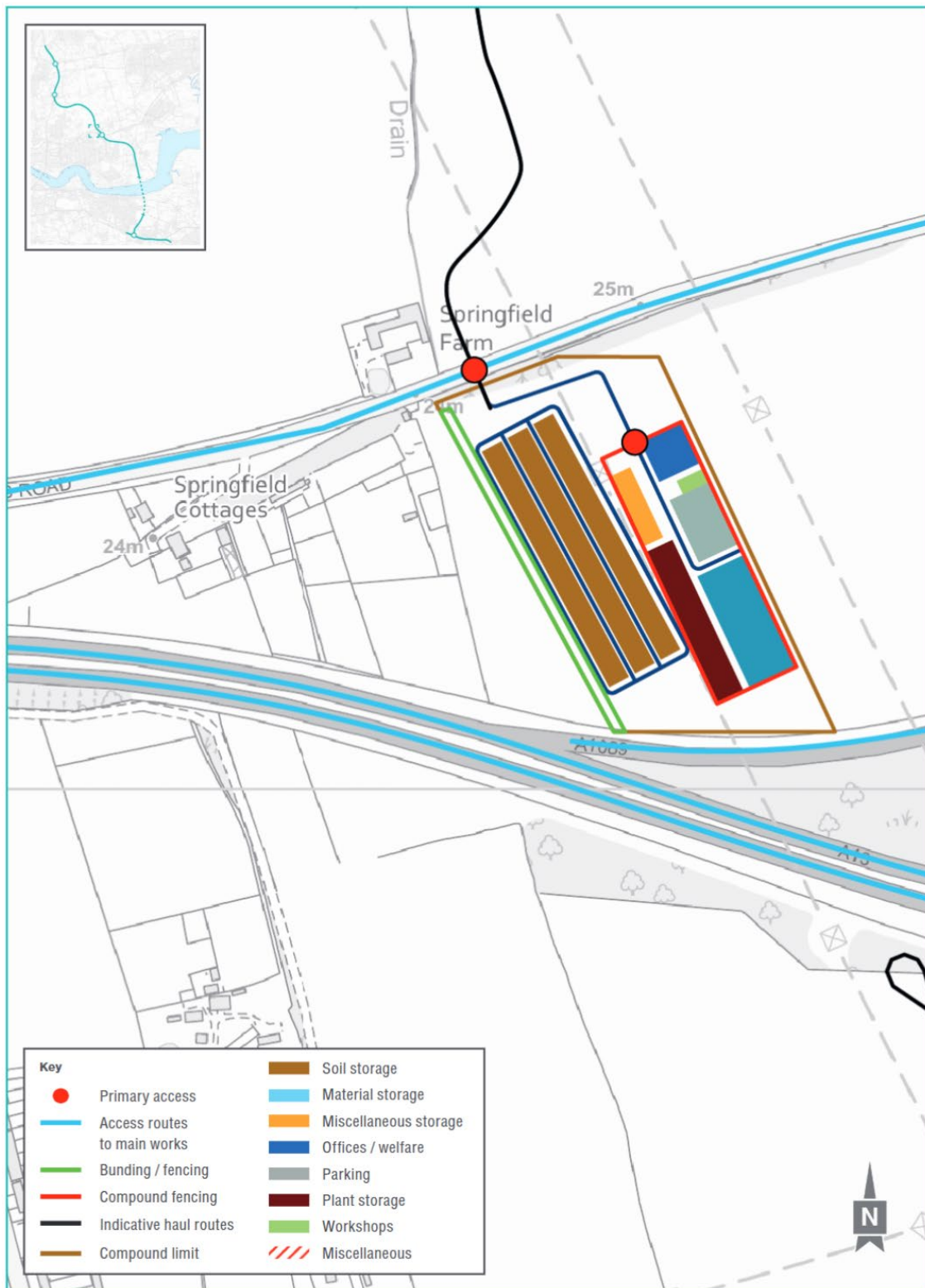
Plate 1.11 Indicative layout for Stifford Clays Road compound West
