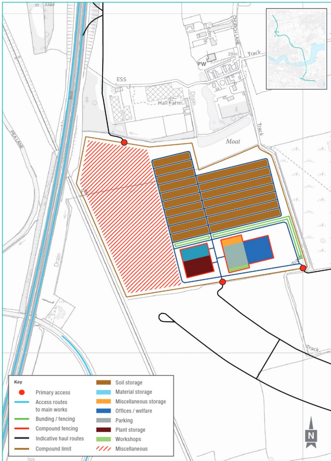
Plate 1.15 Indicative layout for M25 compound
