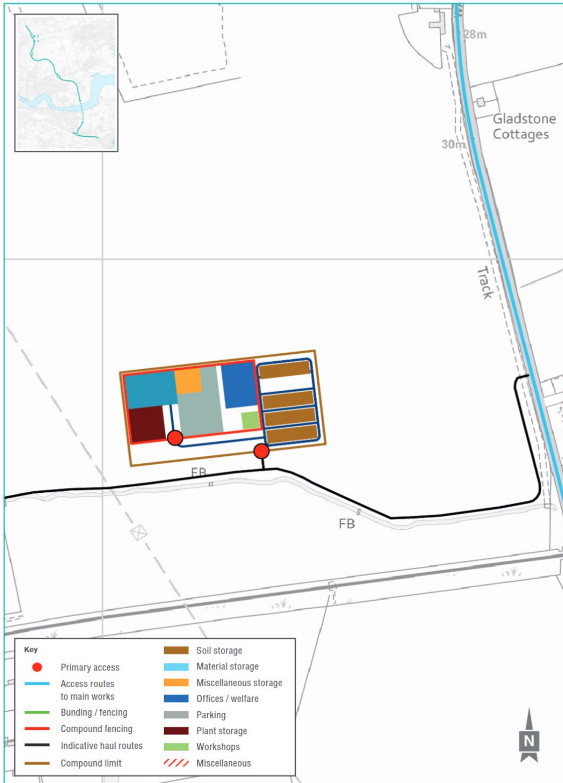
Plate 1.17 Indicative layout for Warley Street compound
