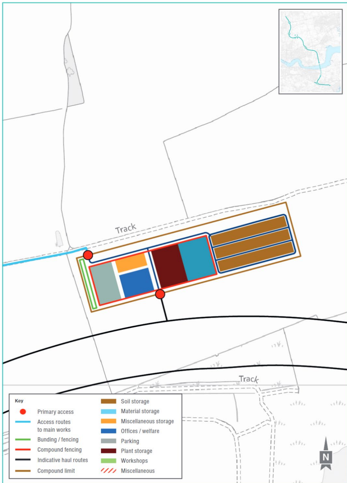
Plate 1.14 Indicative layout for Medebridge compound
