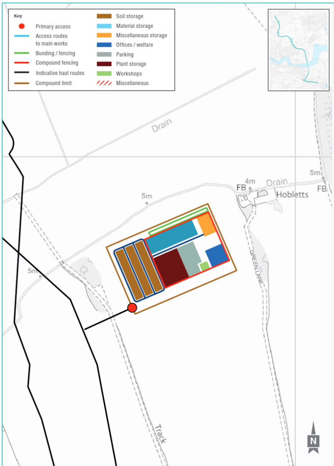
Plate 1.13 Indicative layout for Mardyke compound
