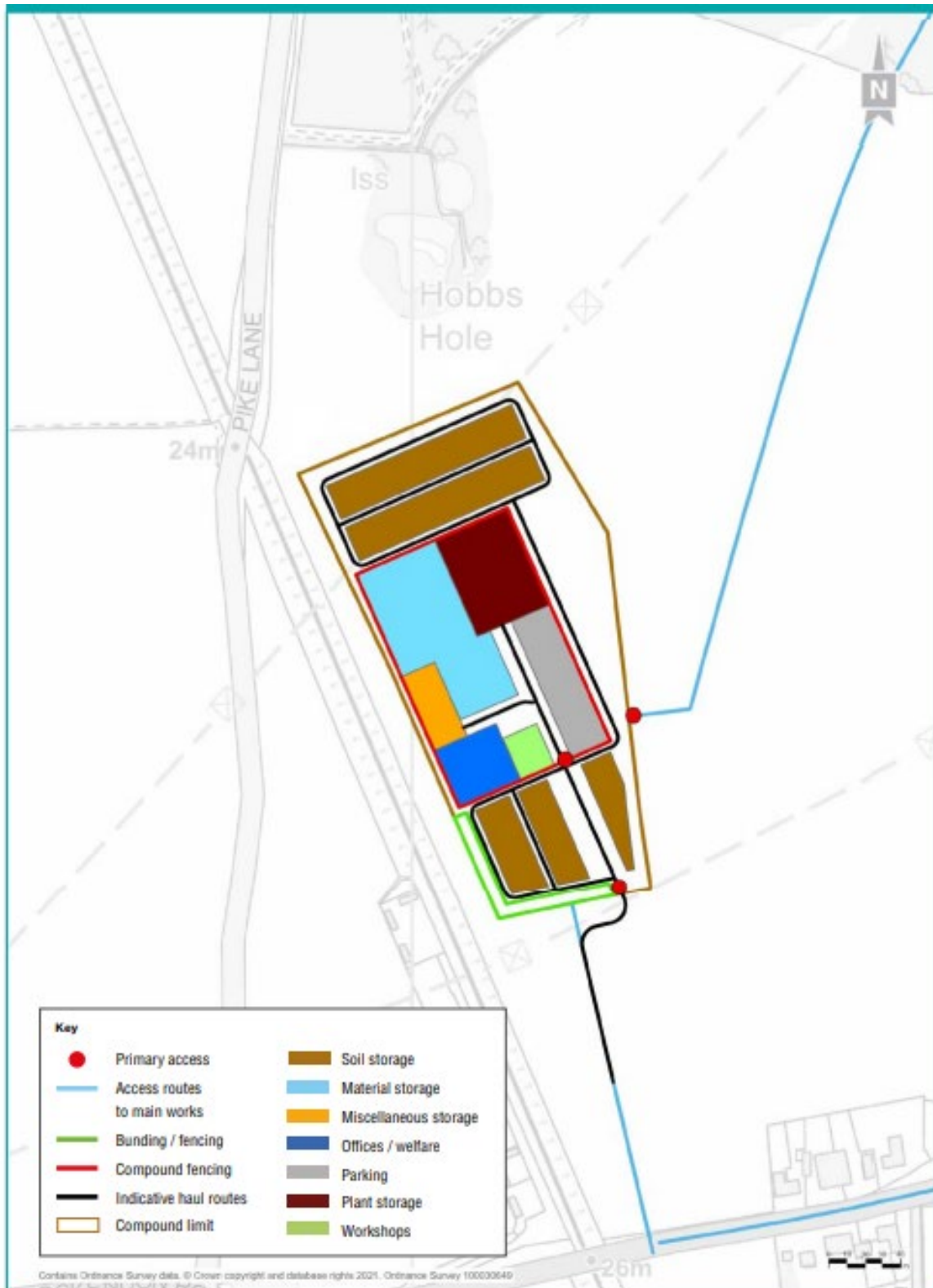
Plate 1.16 Indicative layout for Ockendon Road compound
