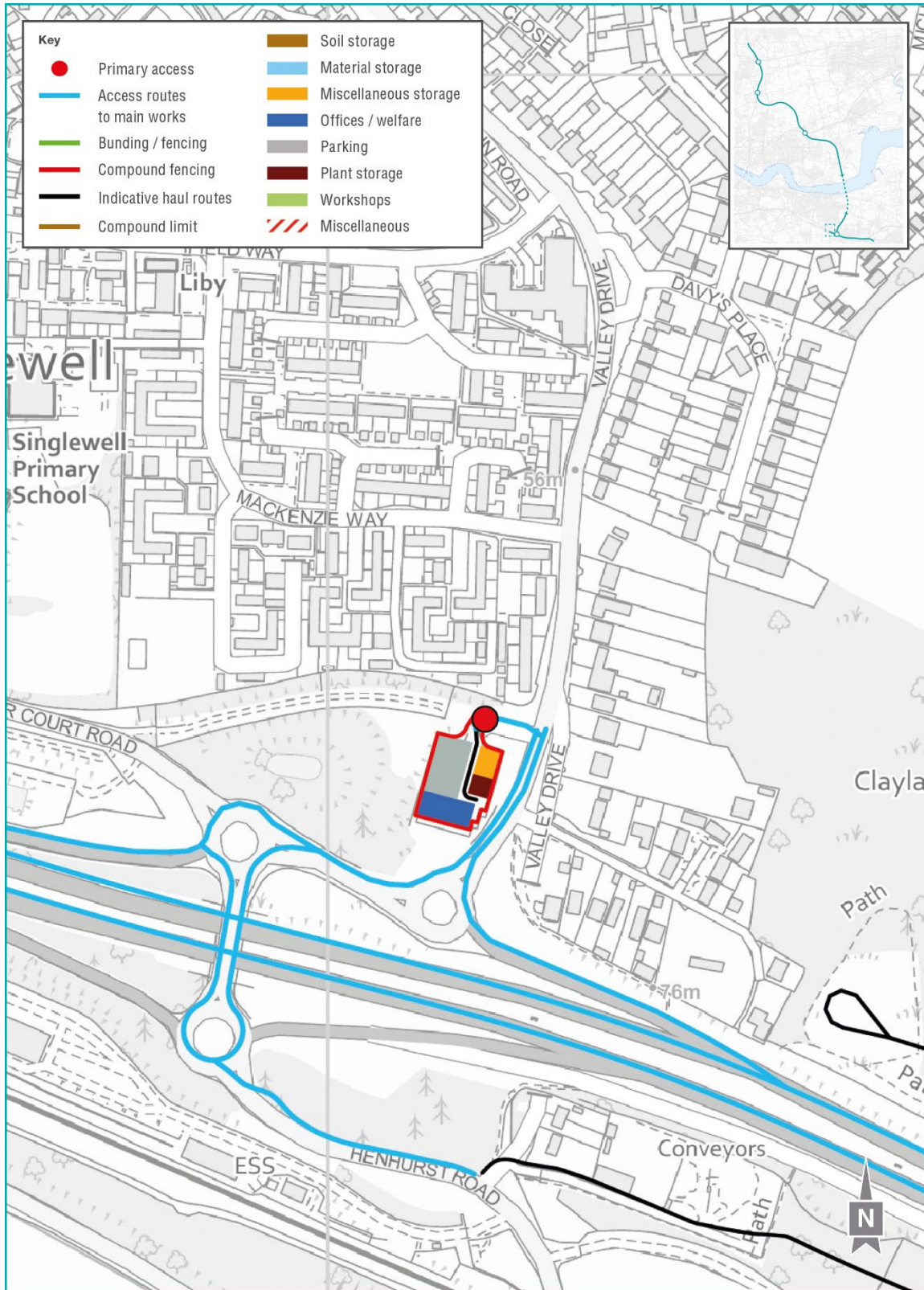
Plate 1.1 Indicative layout for Marling Cross compound
